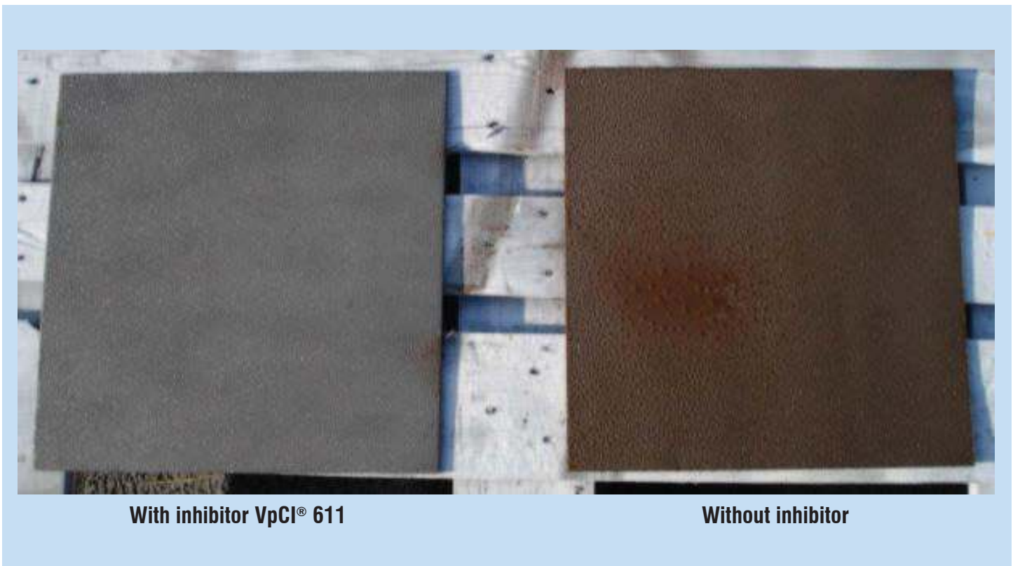
Figure 11. Efficiency testing of corrosion inhibitors in wet blasting process, NCP shipyard, Šibenik
